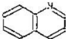
Kinolin
